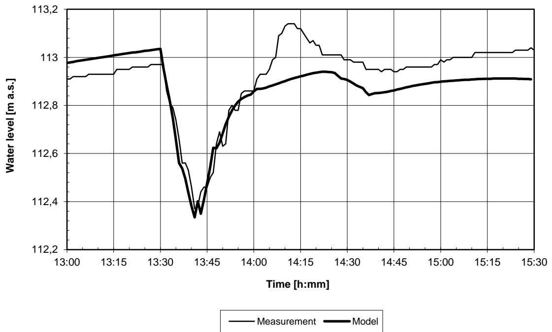
Fig. 8 Comparing water level measurements to results from model
