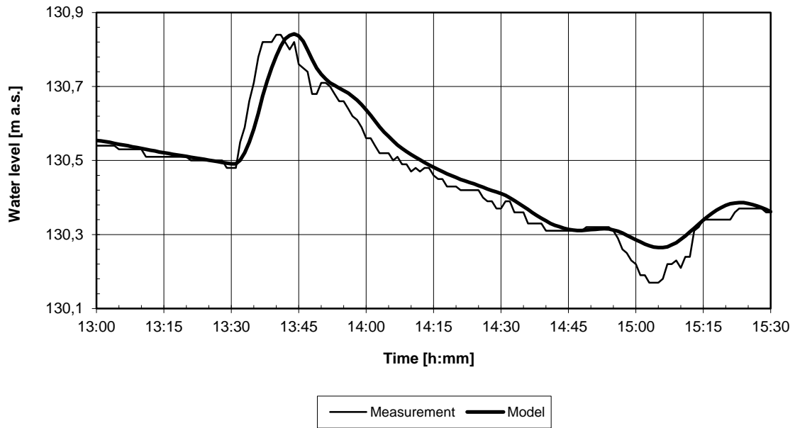
Fig. 7 Comparing water level measurements to results from model
