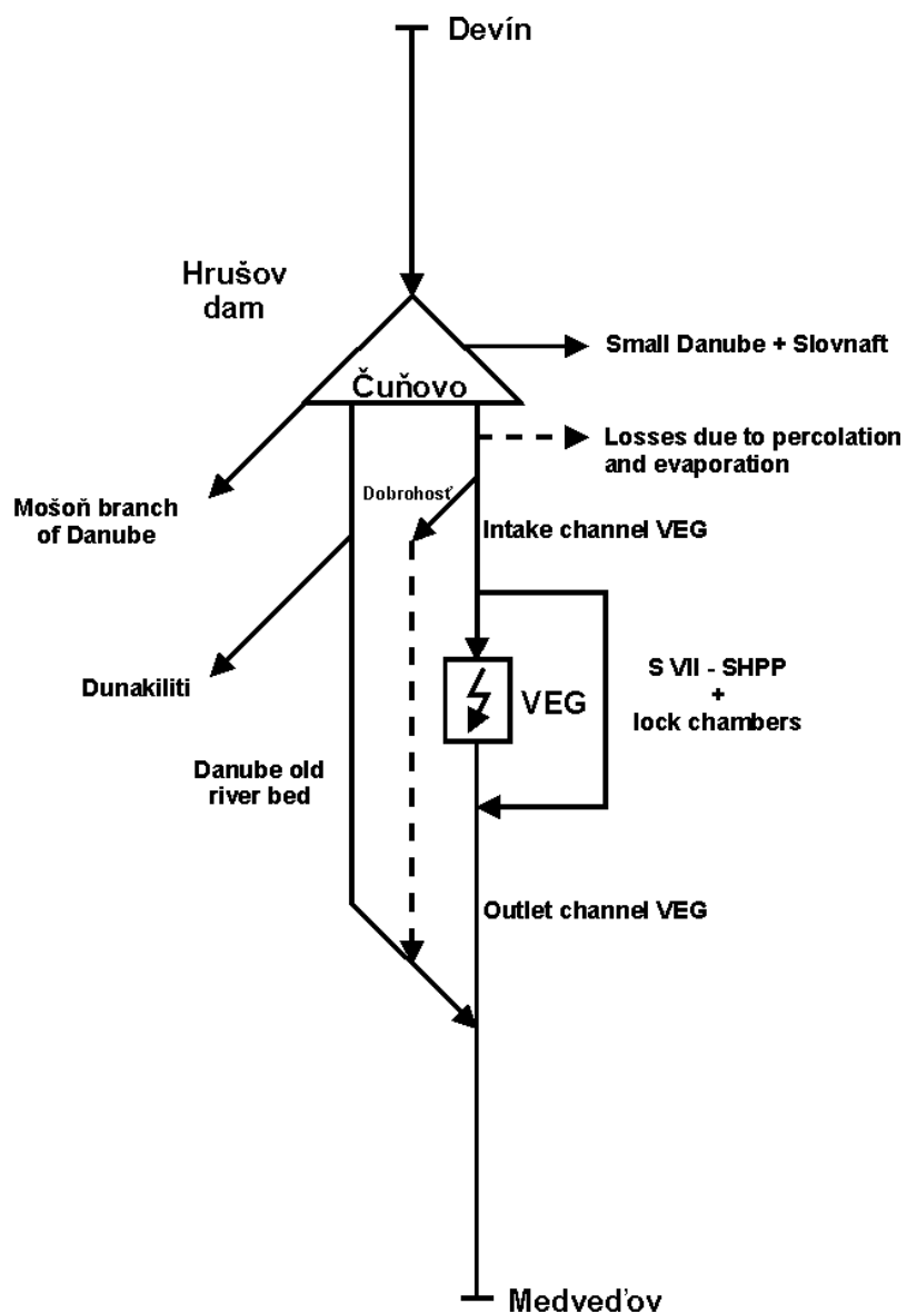
Fig. 4 Scheme of water work Gabčíkovo
