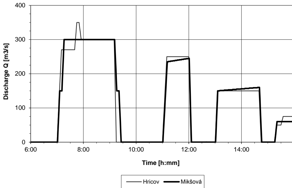
Fig. 2 Time manipulation of discharge
