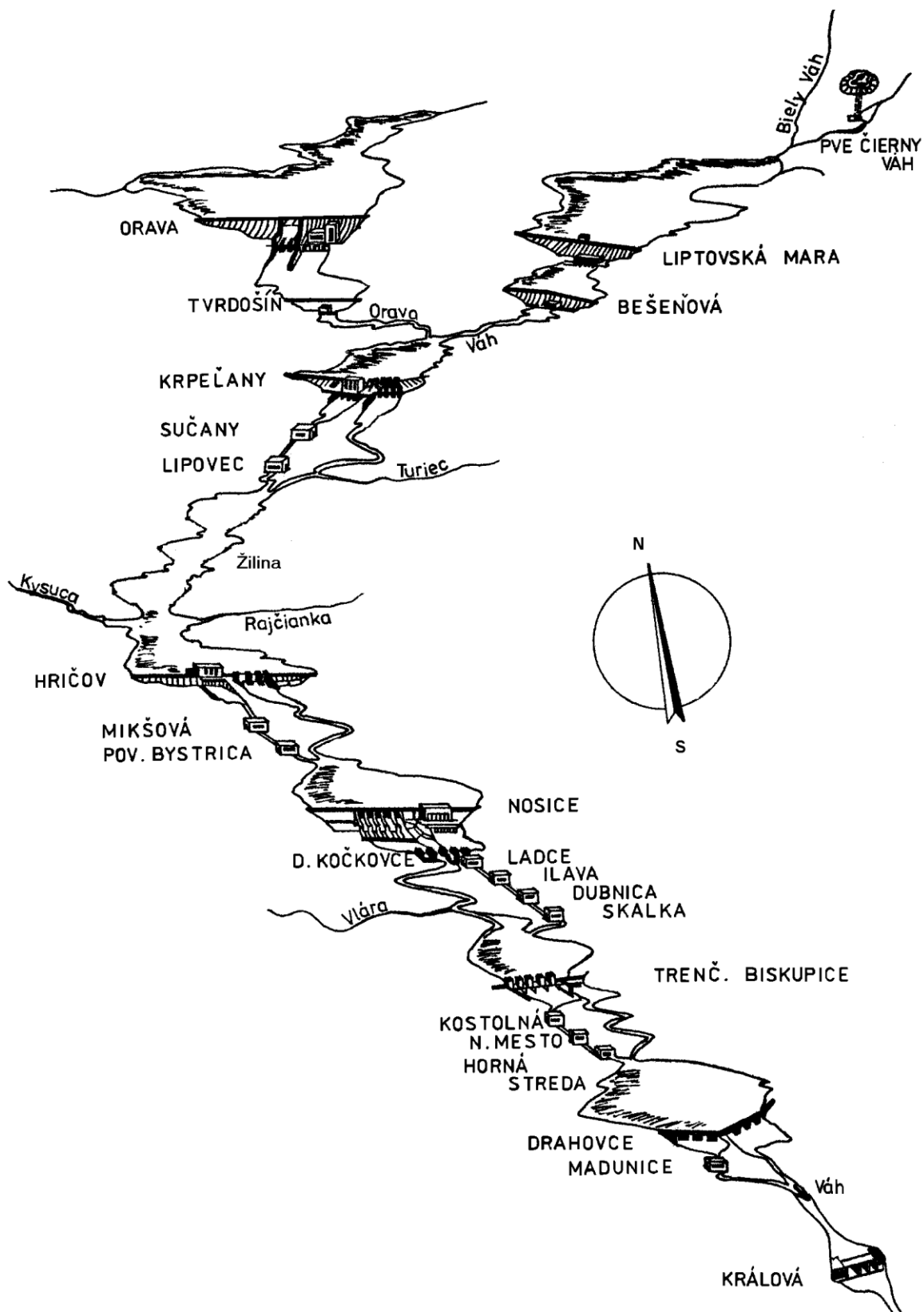
Fig.1 Váh cascade of hydropower plants
