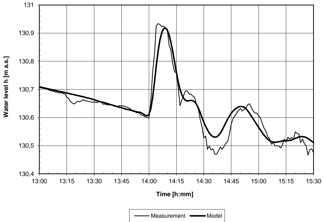
Fig. 6 Comparing water level measurements to results from model
