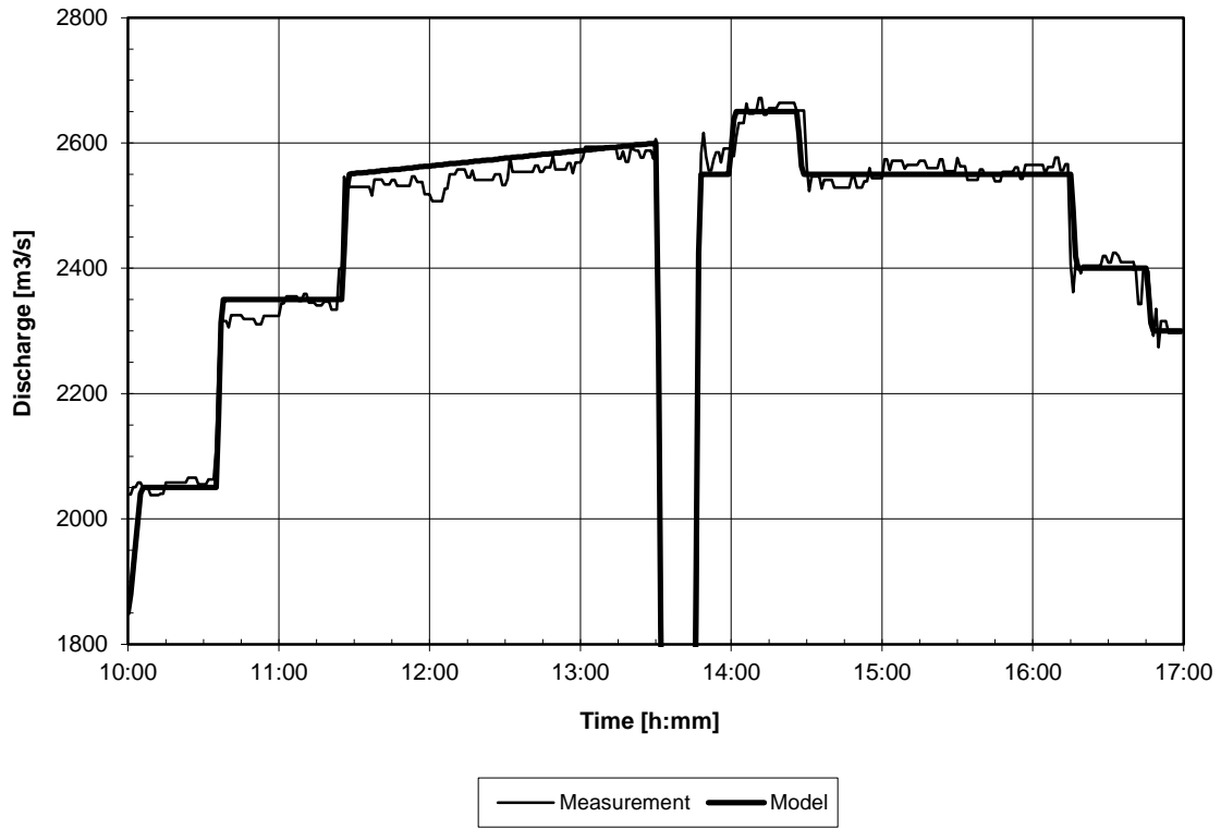
Fig. 5 Time manipulation of discharge
