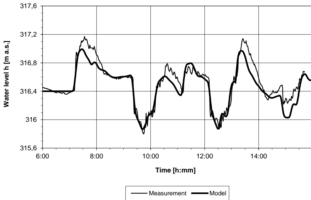
Fig. 3 Comparing water level measurements to results from model
