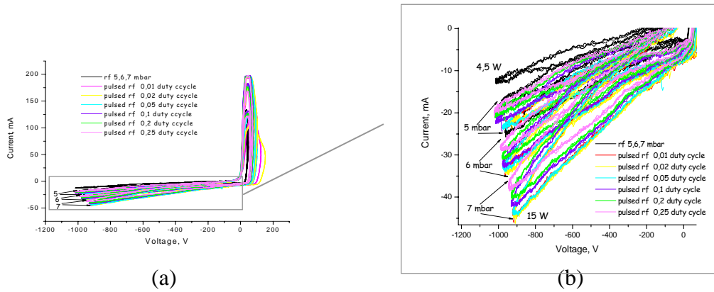
Fig. 5. Voltage-current characteristics of the rf and pulsed-rf discharges
