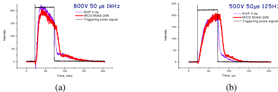
Fig. 2. Emission intensity signal shapes under normal (a) and low (b) conditions
