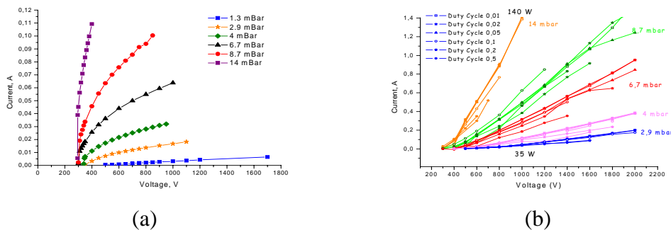
Fig. 4. Voltage-current characteristics of the (a) dc and (b) pulsed dc discharges
