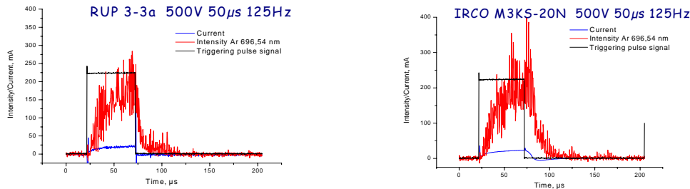
Fig. 3. Emission intensity shapes of single pulses measured under low discharge conditions
