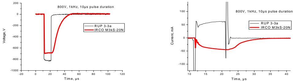
Fig. 1. Voltage and current shapes during the pulse (the current of RUP3-3a is inverted for better presentation)
