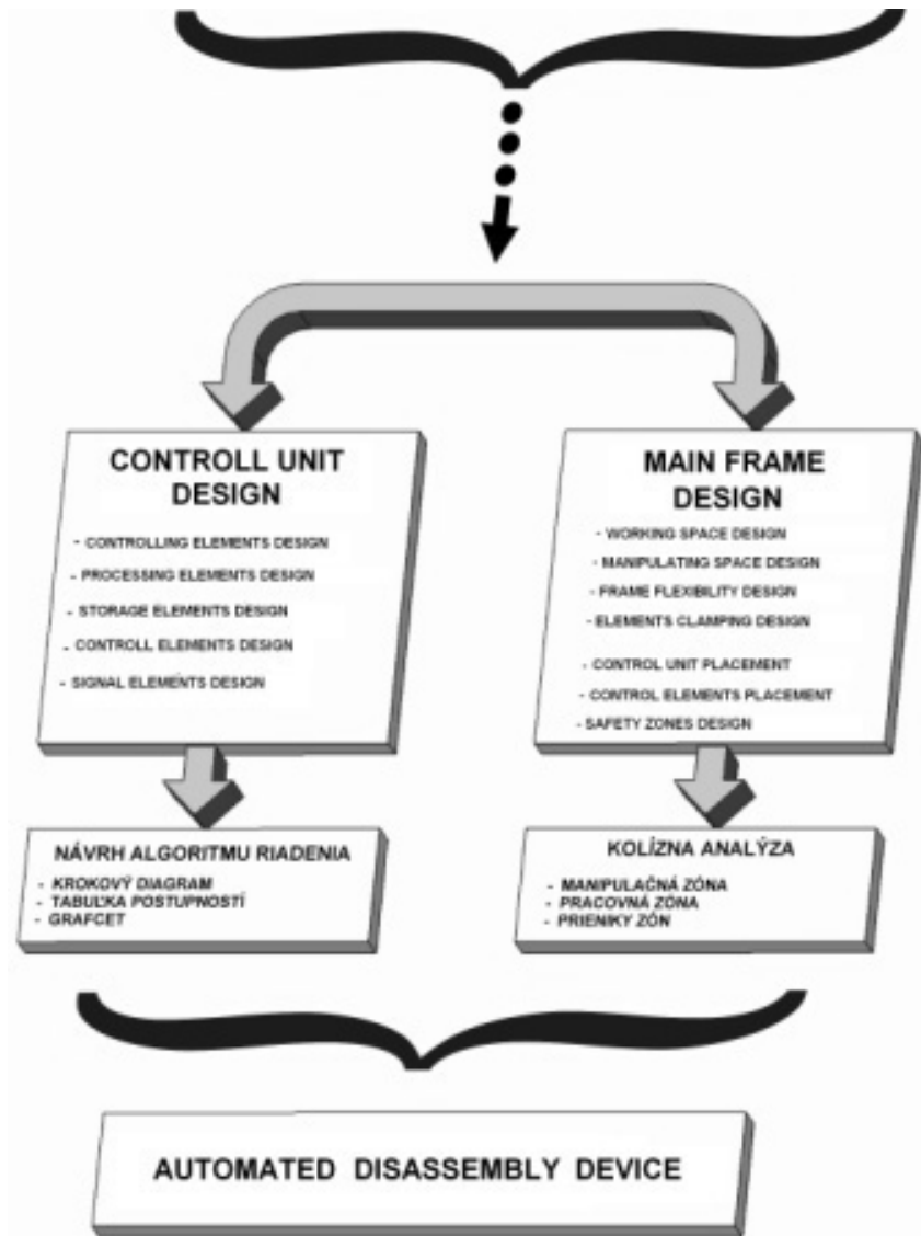
Fig. 6. Automated disassembly device design methodology 2/2
