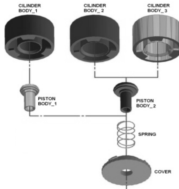
Fig. 1. Assembly process of pneumatic actuator
