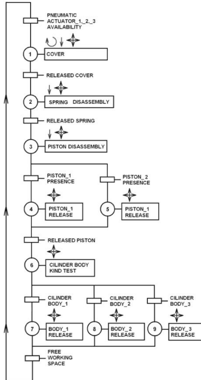
Fig. 4. Supplemented step diagram
