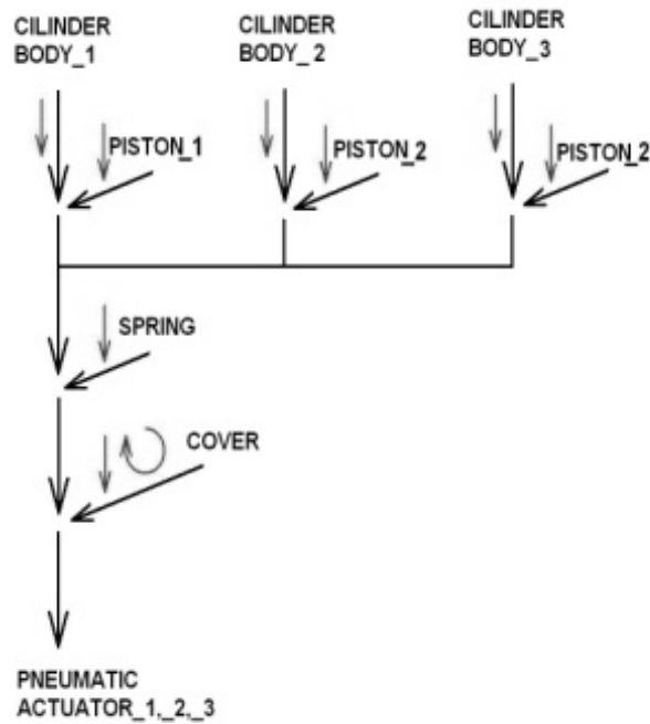
Fig. 2. Step diagram for assembly of pneumatic actuator
